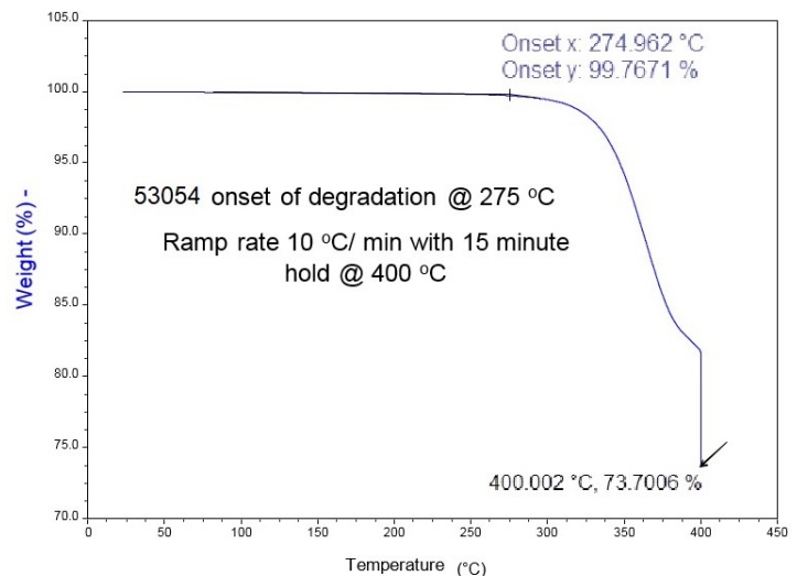
Thermogravimetric Analysis of AOS 340 LR - 53054
